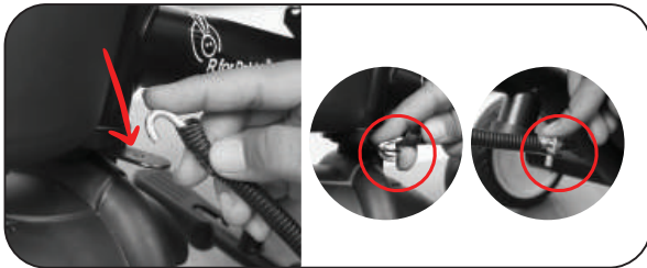
21. Insert the hook shaped rod in front just above the mudguard and tighten it using the nut in backside. Make sure you install the same on left side.
